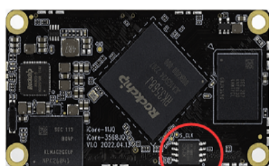
3 SPI Nor
