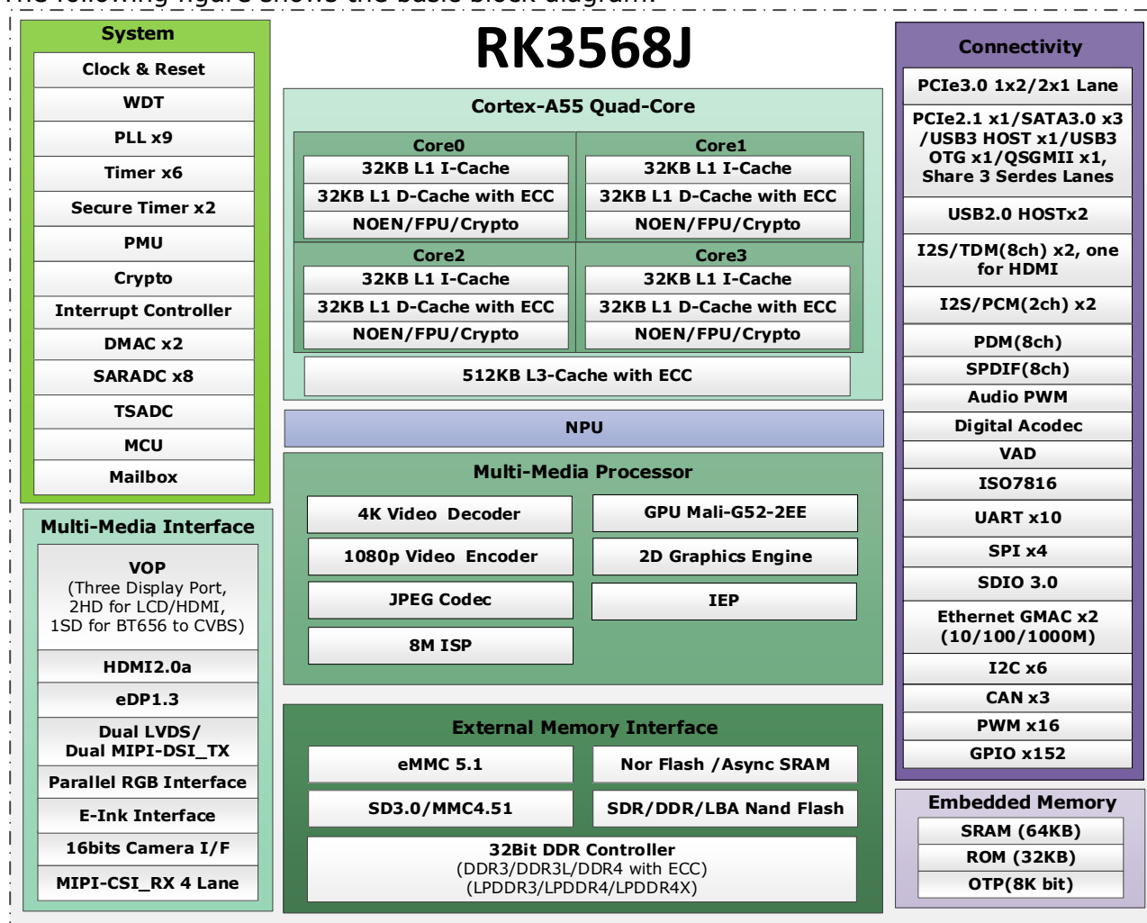
Fig.1-1 Block Diagram
